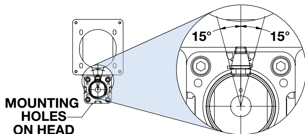
Z12 ZERK ORIENTATION
