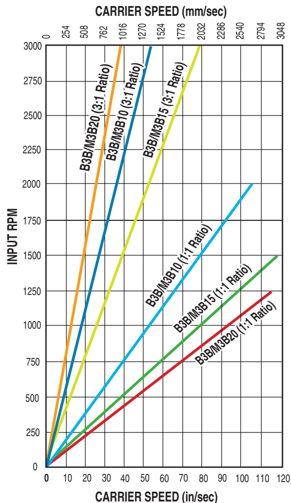
BELT SPEED FOR B3B/M3B ACTUATORS
