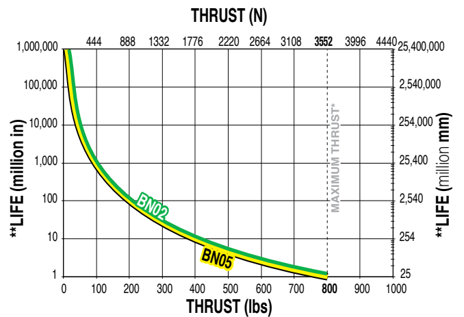
MXE40: Life: Ball Screws
