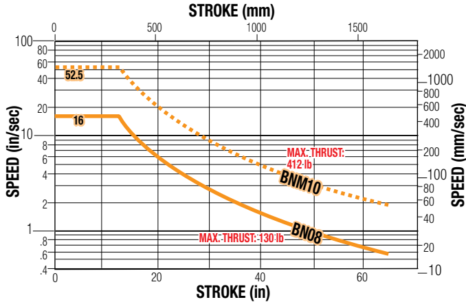
MXE40: Critical Speed: Ball Screw
